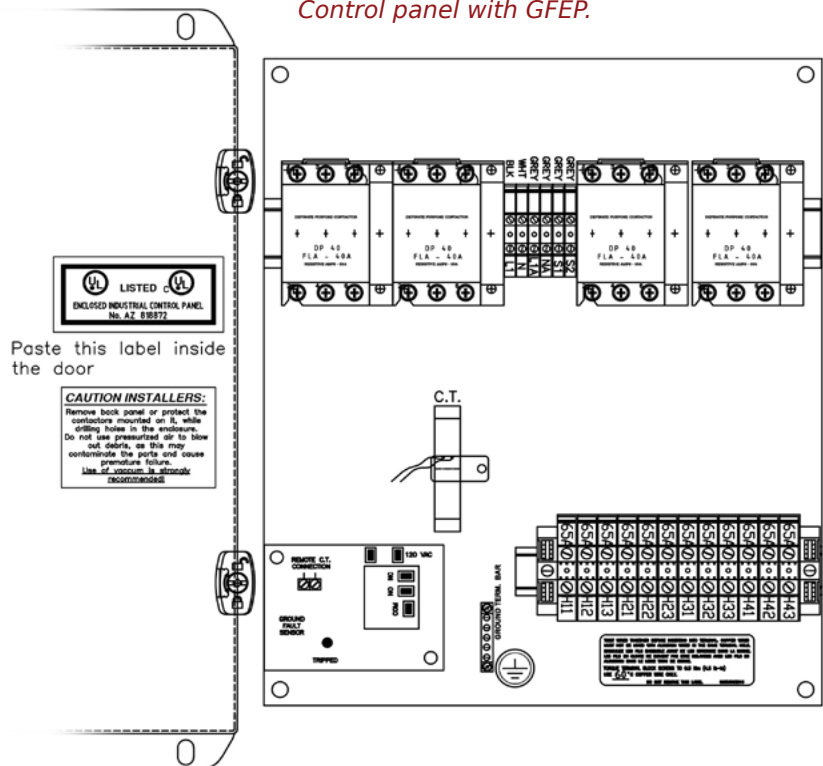
Control panel with GFEP.
