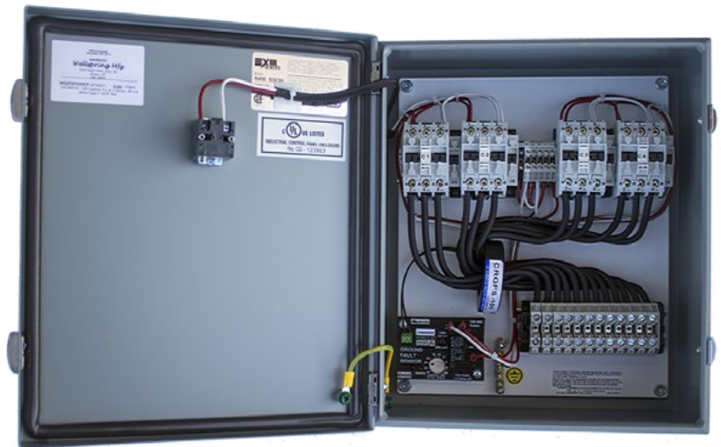
Control panel with GFEP.
